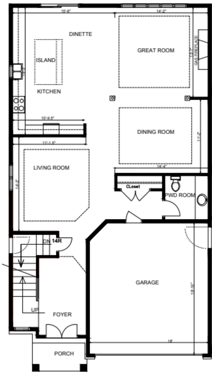
GROUND FLOOR 1293 s.f. TYPE "A"
